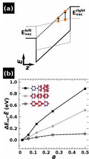
Figure 6. (a) Simplified sketch of the electron electrostatic energy across a SAM of 3N molecules at low (dashed gray) and high (solid black) packing density. The orange symbols illustrate how the energy is changed differently at different positions in the well upon increasing the SAM packing density. (b) Energetic shifts of the HOMO (black squares), HOMO-1 (gray circles), and LUMO (black diamonds) derived bands in a SAM of 3N molecules upon increasing the SAM packing density \theta , aligned at the average electrostatic energy \bar{E} = (E_{\text{vac}}^{\text{left}} + E_{\text{vac}}^{\text{right}})/2 (cf. Figure 3a). The energies are determined from the onsets of the respective peaks in the DOS.
